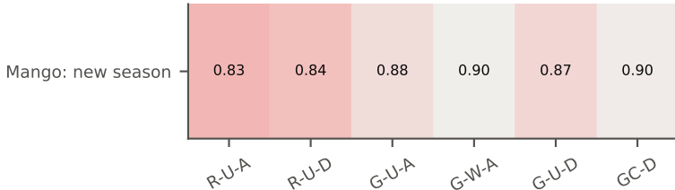
(a) Coverage (colour: deviation from 0.90)
