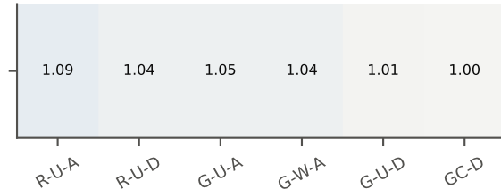
(b) Interval score relative to GC-D
