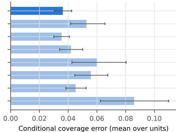
R2 cluster-out
