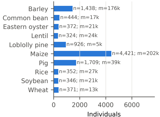
a Datasets (EasyGeSe)
