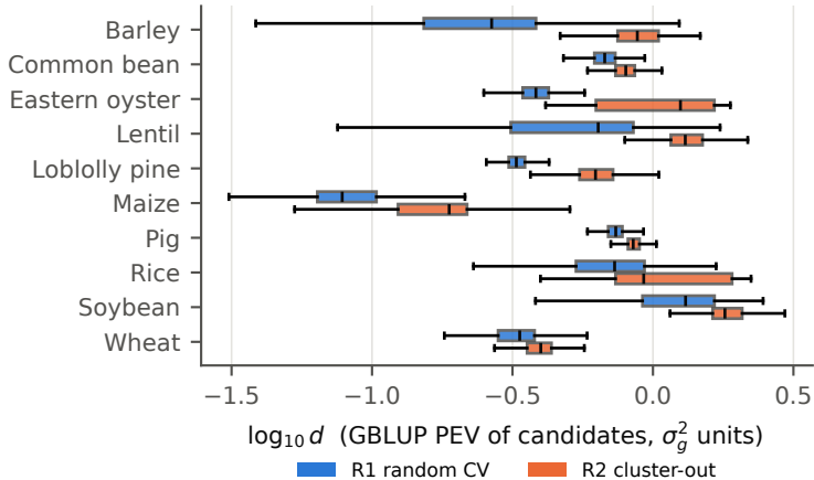
b Relatedness covariate of test candidates
