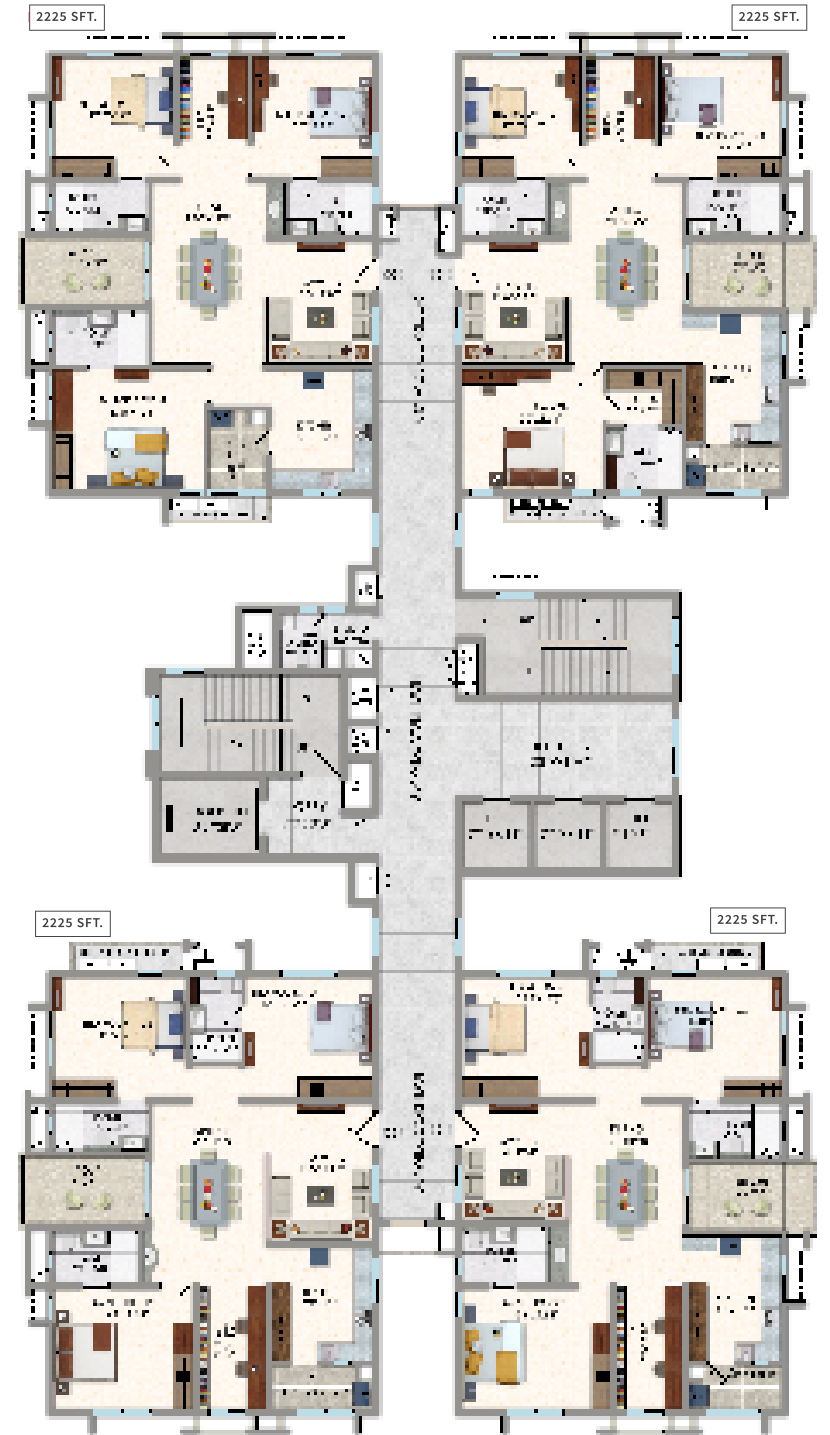
Typical Floor Plan - Block C
