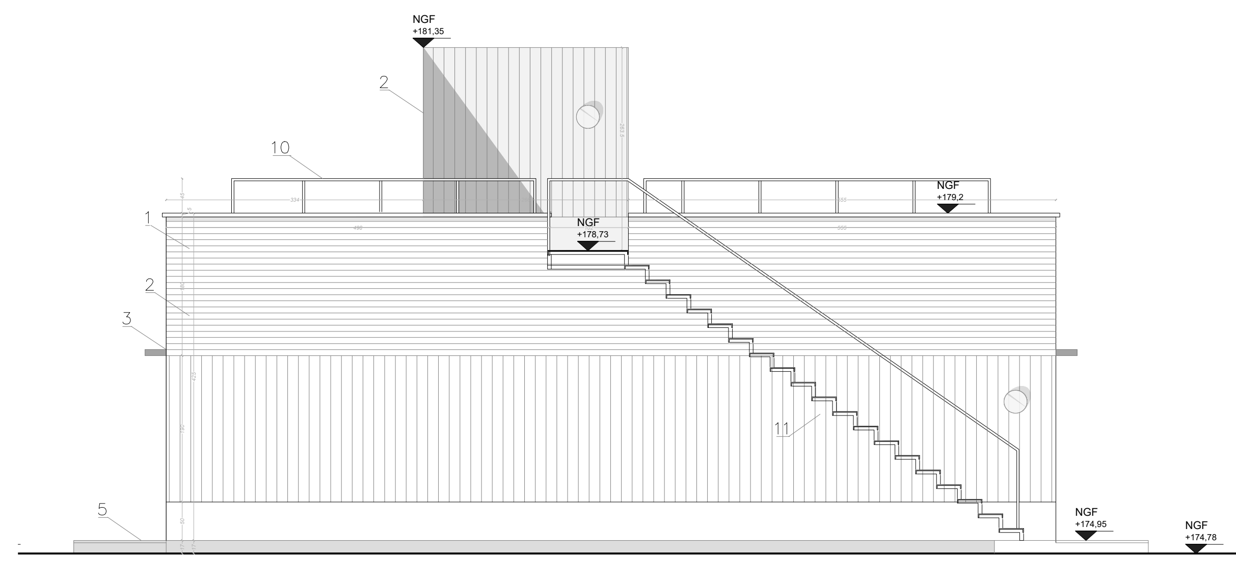
Elevation 3F – 1/100
