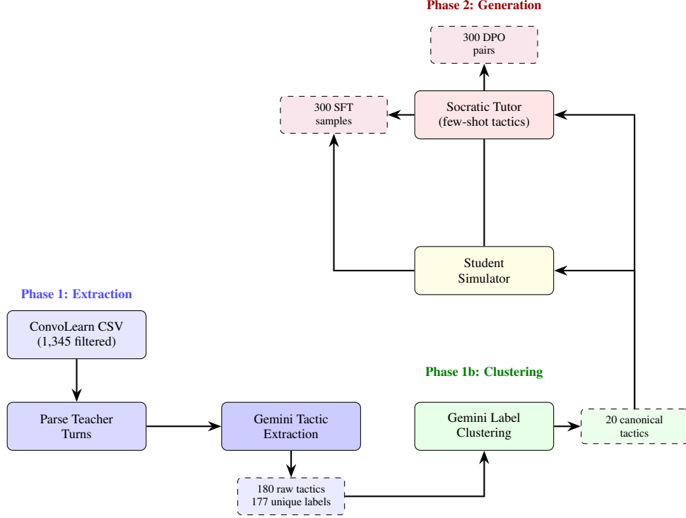
Figure 4: Three-phase synthetic data pipeline. Phase 1 extracts pedagogical tactics from ConvoLearn teacher turns. Phase 1b consolidates 177 noisy labels into 20 canonical tactics. Phase 2 uses dual-agent simulation (student simulator + tactic-guided Socratic tutor) to generate DSA-grounded SFT dialogues and DPO preference pairs.
