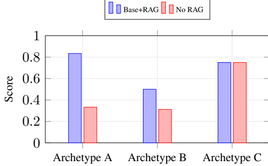
Figure 6: E1 per-archetype scores. Base+RAG dominates on Archetypes A and B (gap detection) while maintaining competitive performance on C (teaching).
