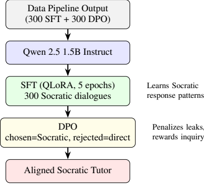
Figure 5: Two-stage alignment pipeline using synthetic data from the three-phase data pipeline (§3.2).
