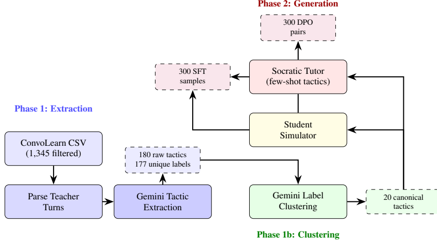
Figure 4: Three-phase synthetic data pipeline. Phase 1 extracts pedagogical tactics from ConvoLearn teacher turns. Phase 1b consolidates 177 noisy labels into 20 canonical tactics. Phase 2 uses dual-agent simulation (student simulator + tactic-guided Socratic tutor) to generate DSA-grounded SFT dialogues and DPO preference pairs.
