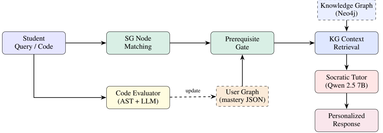
Figure 1: End-to-end system architecture. A student query is mapped to a Skeleton Graph node, prerequisite-gated against the student’s mastery state, enriched with KG context (definitions, misconceptions, analogy bridges), and passed to the Socratic tutor. Code submissions follow a parallel path through the hybrid evaluator, which updates mastery scores.
