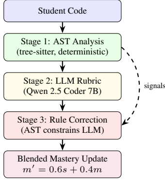
Figure 3: The hybrid code evaluation pipeline. AST analysis provides ground-truth structural signals that constrain LLM scoring.
