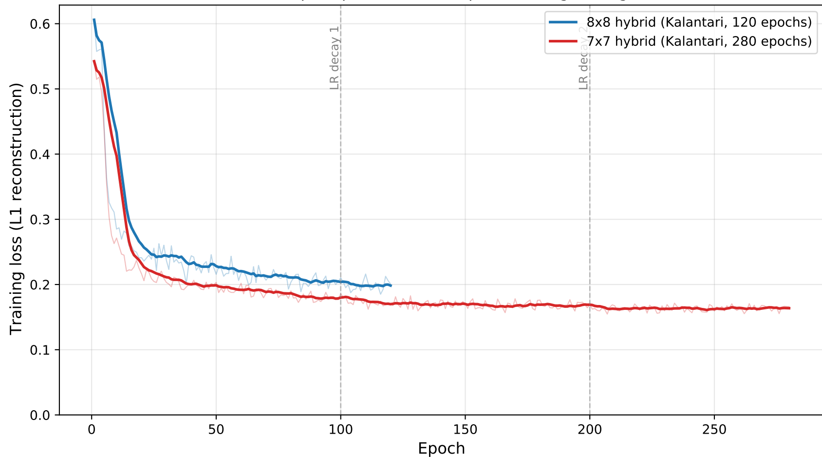
Hybrid model training loss over epochs (faded: per-epoch, bold: 10-epoch moving average)
