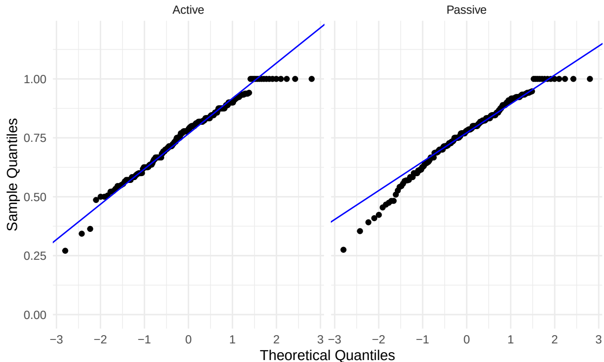
Q-Q Plots: IR Memorability by Sentence Voice Checking for Normality across Active and Passive Voices
