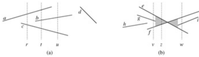
Figure 33.4: The ordering among line segments at various vertical sweep lines. (a) We have a >_r c , a >_t b , b >_t c , a >_u c , and b >_u c . Segment d is comparable with no other segment shown. (b) When segments e and f intersect, their orders are reversed: we have e >_v f but f >_w e . Any sweep line (such as z ) that passes through the shaded region has e and f consecutive in its total order.
