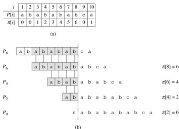
Figure 32.11: An illustration of Lemma 32.5 for the pattern P = \text{ababababca} and q = 8 . (a) The \pi function for the given pattern. Since \pi[8] = 6 , \pi[6] = 4 , \pi[4] = 2 , and \pi[2] = 0 , by iterating \pi we obtain \pi^*[8] = \{6, 4, 2, 0\} . (b) We slide the template containing the pattern P to the right and note when some prefix P_k of P matches up with some proper suffix of P_8 ; this happens for k = 6, 4, 2 , and 0 . In the figure, the first row gives P , and the dotted vertical line is drawn just after P_8 . Successive rows show all the shifts of P that cause some prefix P_k of P to match some suffix of P_8 . Successfully matched characters are shown shaded. Vertical lines connect aligned matching characters. Thus, \{k : k < q \text{ and } P_k \sqsubset P_q\} = \{6, 4, 2, 0\} . The lemma claims that \pi^*[q] = \{k : k < q \text{ and } P_k \sqsubset P_q\} for all q .
