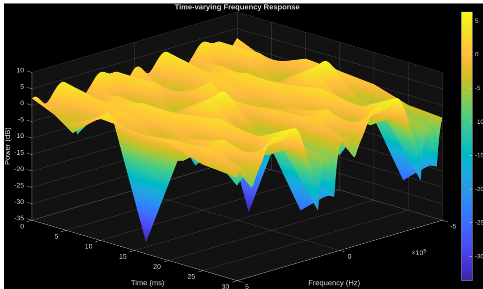
Figure 18: 3-D Doppler channel response.
