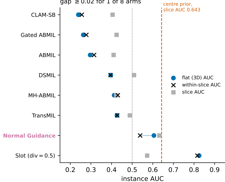
B. Flat AUC is within-slice AUC gap \geq 0.02 for 1 of 8 arms
