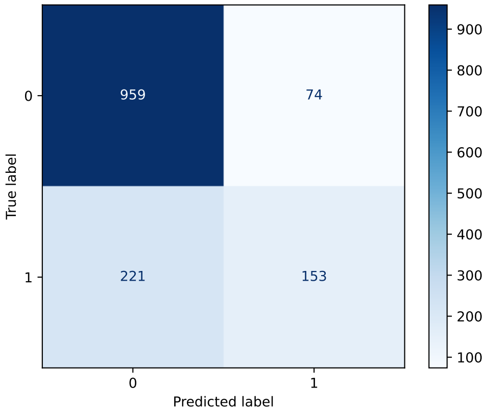
Model Confusion Matrix
