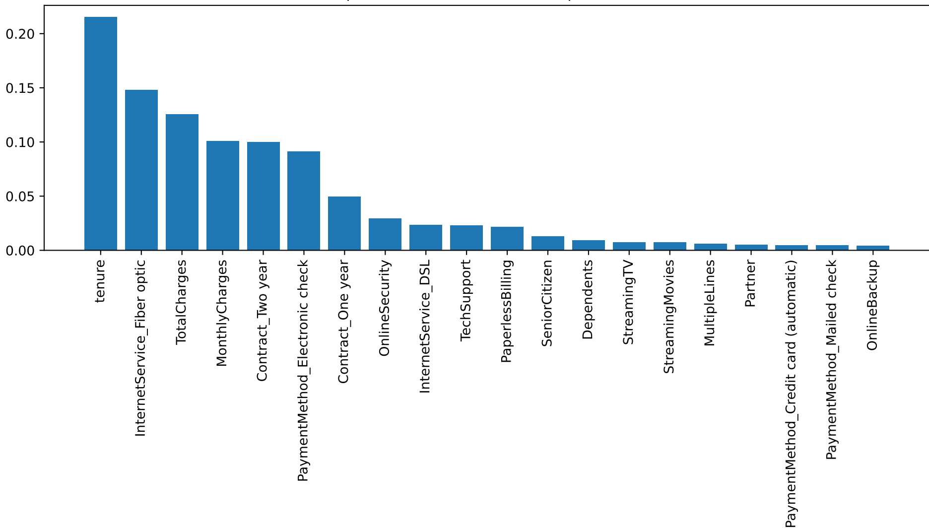
Top Churn Drivers (Feature Importance)
