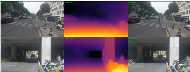
Fig. 3. Visualization of stabilization and depth estimation. For each scene: (Left) original frame, (Middle) depth map predicted by MiDaS, and (Right) stabilized frame using our method. Top and bottom rows represent different scenes. The stabilized output shows improved spatial alignment and smoother visual consistency.
