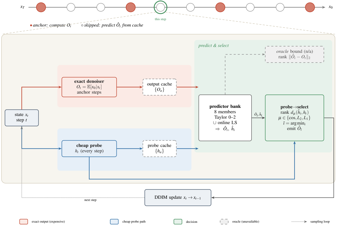
Figure 1: Architecture of the exact-residual testbed and the probe-then-select mechanism. Because the prior is a Gaussian mixture, the true denoiser output O_t (red, “expensive”) is available in closed form, and a cheap hard-assignment probe h_t (blue) plays the role of a first-layer readout. At a skipped step the predictor bank extrapolates the cached outputs and probes; the selector ranks predictors by a proxy distance on the probe and applies the winner’s output. The oracle (dashed) ranks by the true output error and is never deployable—it bounds how much any proxy could gain.
