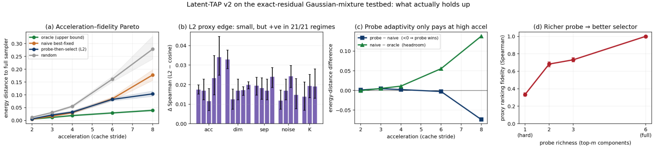
Figure 4: (a) Acceleration–fidelity trade-off: probe-then-select tracks the naive best-fixed predictor until high stride, where it separates toward the oracle. (b) The L_2 proxy advantage over cosine is small but positive in all 21 regimes, widening with acceleration and noise. (c) Probe adaptivity is beneficial only at aggressive acceleration (probe–naive crosses below 0 at stride 8), where the selection headroom (naive–oracle) is largest. (d) Proxy fidelity increases monotonically with probe richness, from a shallow hard probe (0.33) to the full output (1.0); this is the axis along which a trained DiT probe would improve.
