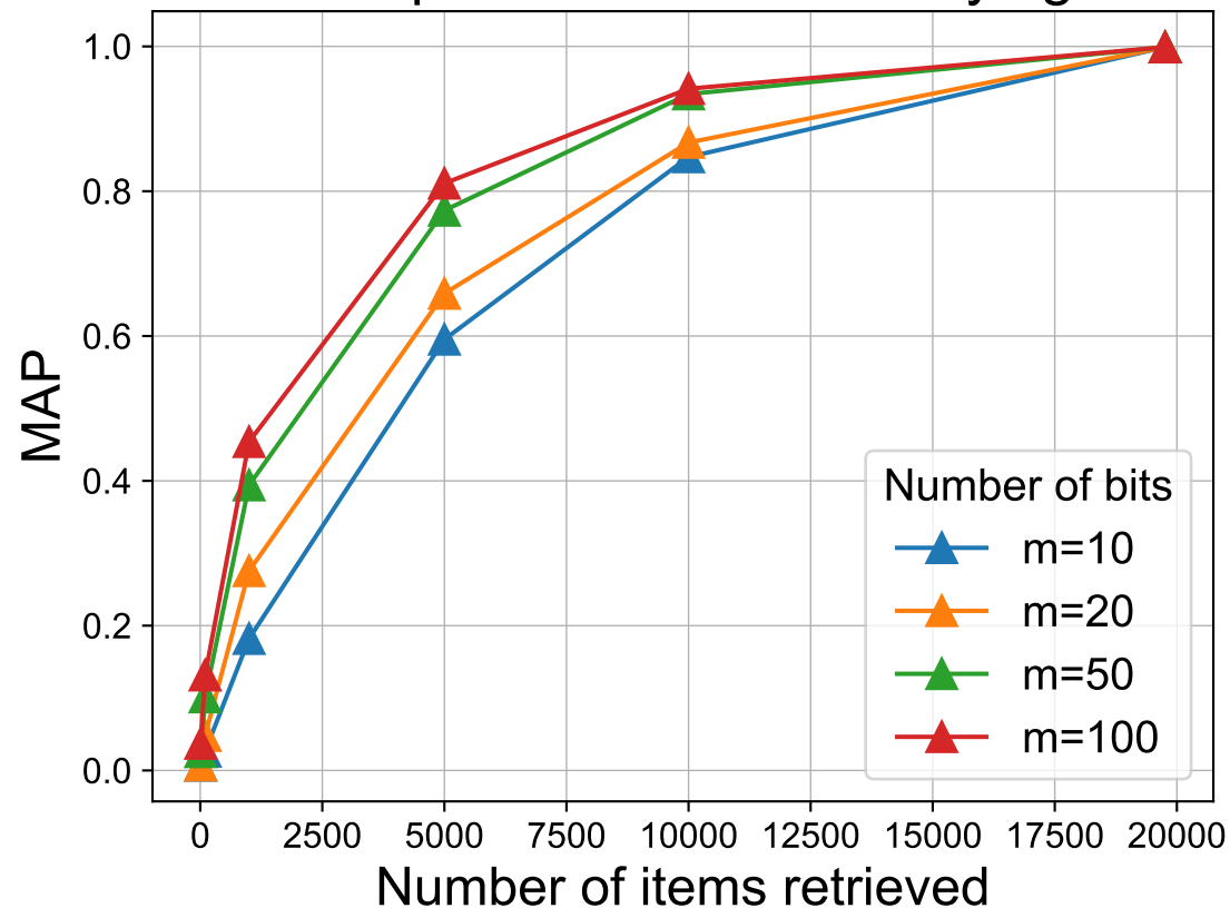
FAISS performance with varying m
