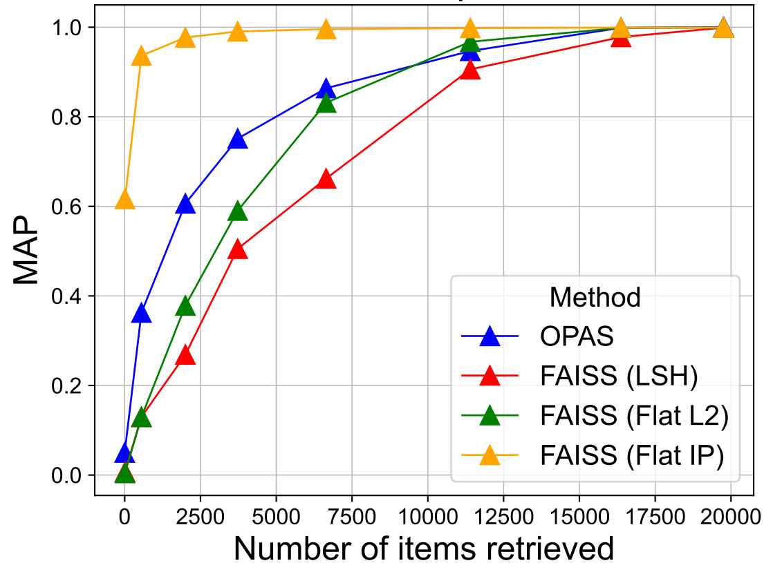
OPAS vs FAISS performance
