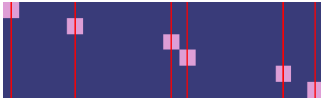
Linear Sum Assignment
