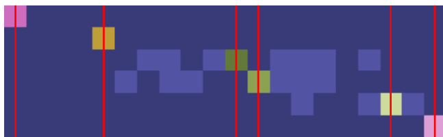
Sinkhorn ( \tau=0.05 )
