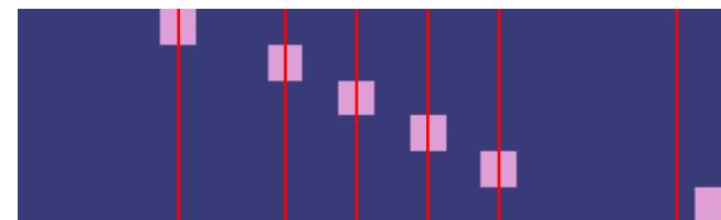
Sinkhorn ( \tau=0.001 )
