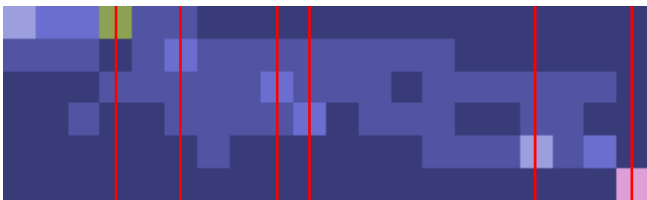
Sinkhorn ( \tau=1 )
