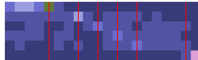
Sinkhorn ( \tau=1 )
