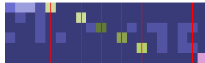
Sinkhorn ( \tau=0.05 )
