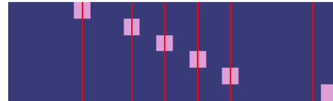
Linear Sum Assignment
