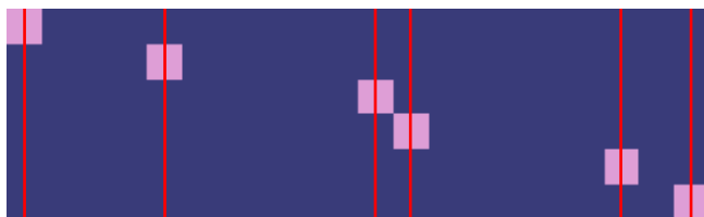
Sinkhorn ( \tau=0.001 )
