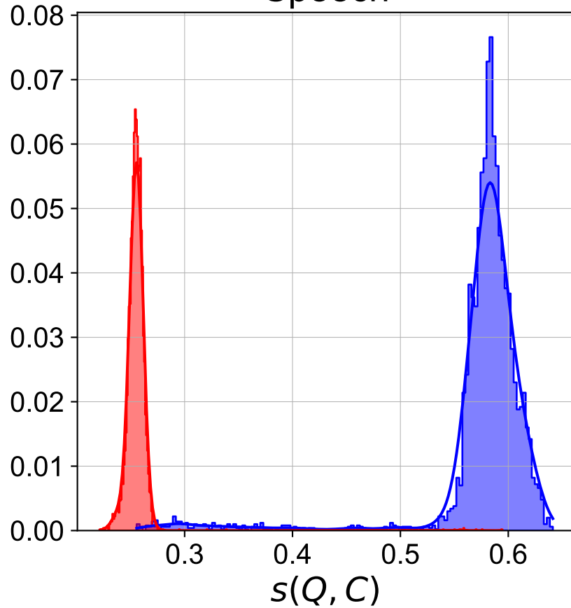
Speech
