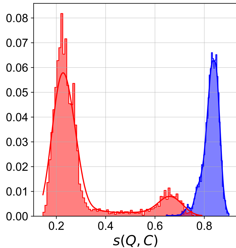
LSUN
