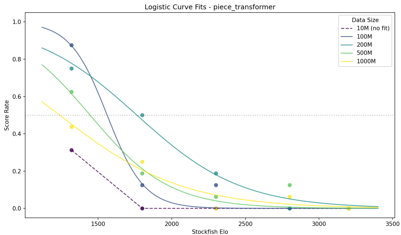
Figure A.30: Logistic Elo fit for Piece Transformer.
