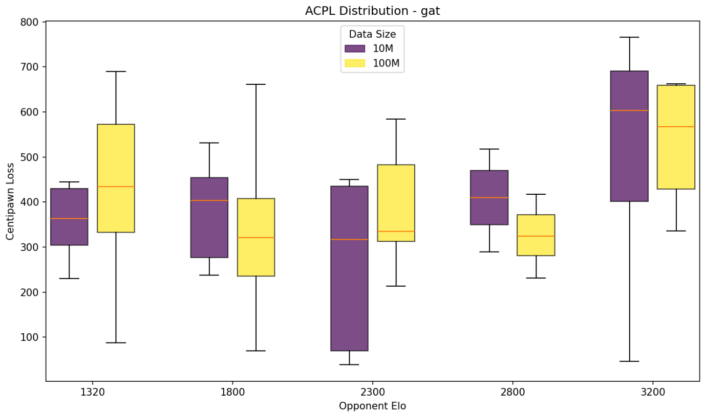
Figure A.34: ACPL distribution for GAT.
