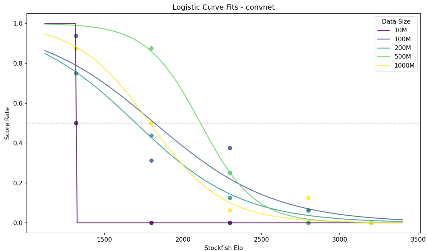
Figure A.27: Logistic Elo fit for ConvNet.
