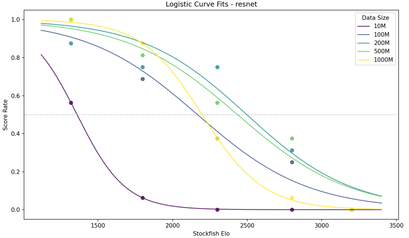
Figure 5.6: Logistic fits for Elo estimation of the ResNet architecture against Stockfish.
