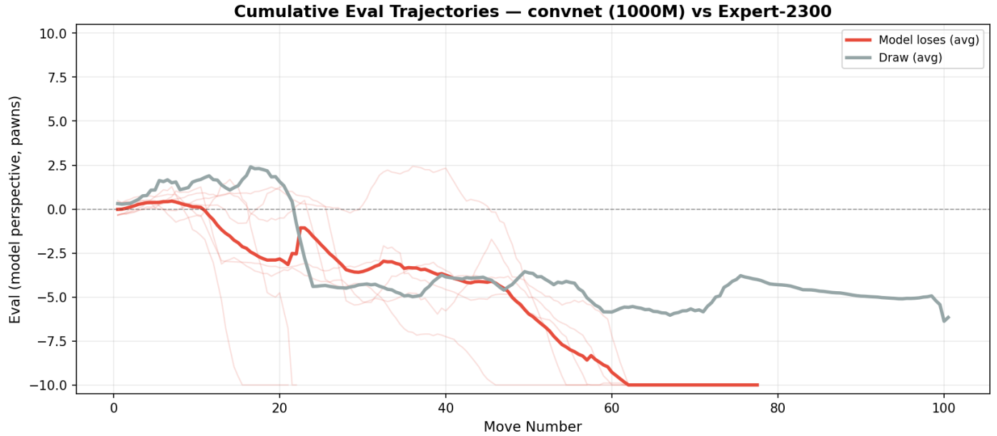
Figure A.4: Cumulative evaluation for ConvNet 1000M against Stockfish 2300.
