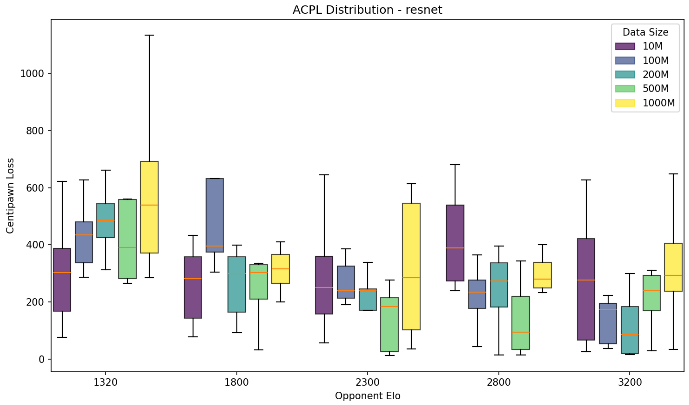
Figure A.37: ACPL distribution for ResNet.
