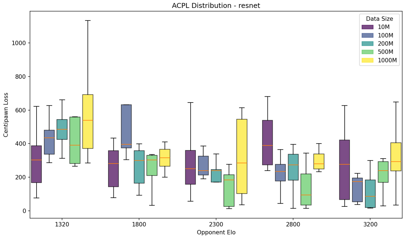
Figure 5.7: Average Centipawn Loss (ACPL) boxplot for ResNet models.
