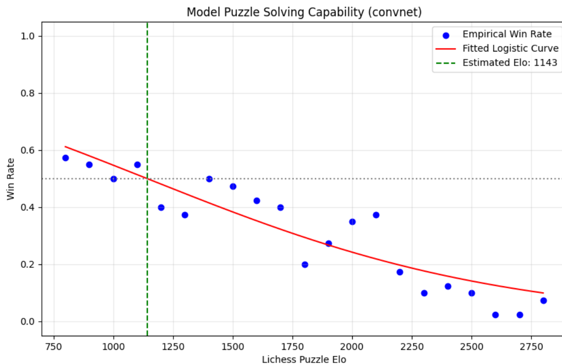
Figure A.39: Puzzle benchmark accuracy for ConvNet 1000M.
