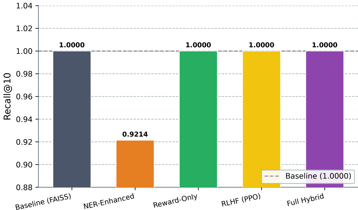
Recall@10: All Methods
