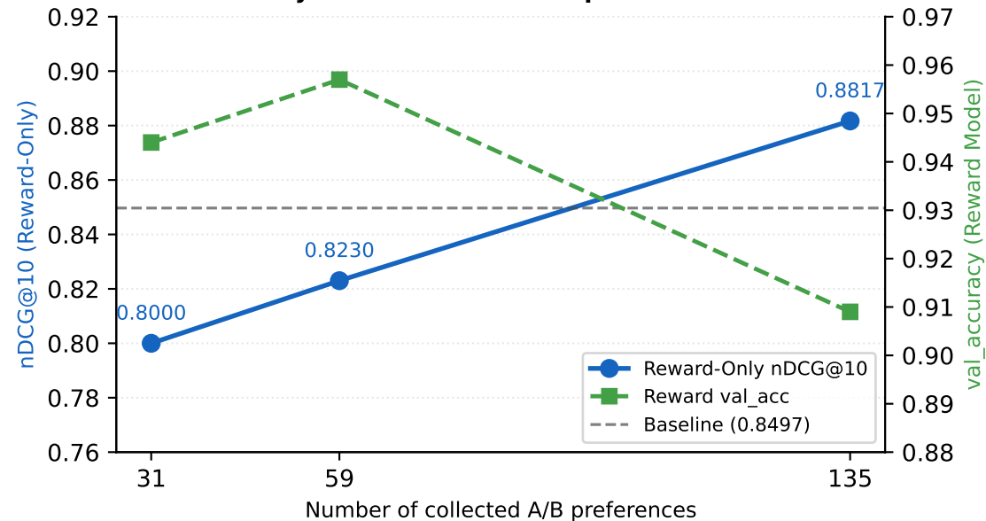
RLHF system evolution with preference data
