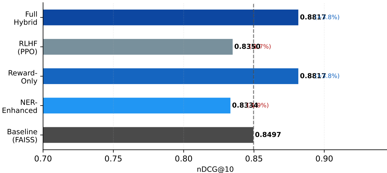
nDCG@10 comparison by ranking method
