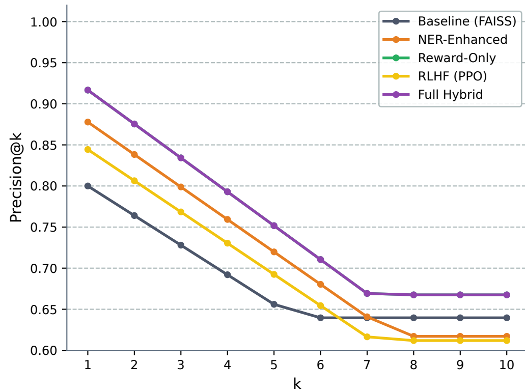
Precision@k vs k
