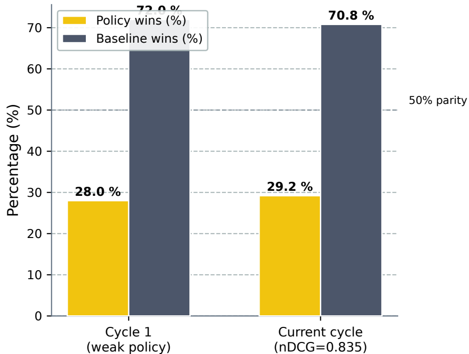
Policy vs Baseline Win Rate Comparison
