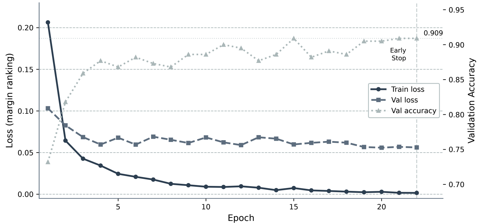
Reward Model Training: Loss and Accuracy Curves
