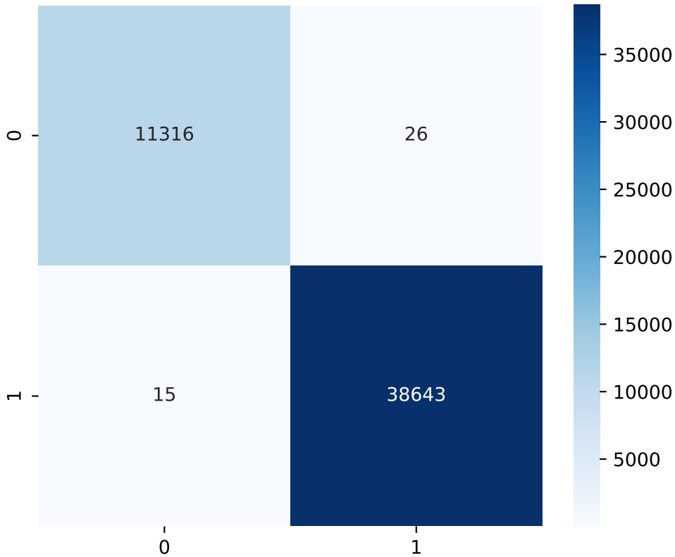
XGBoost - Confusion Matrix
