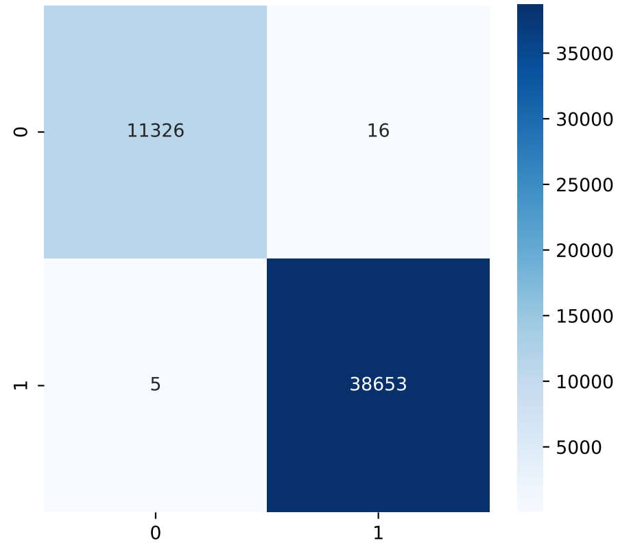
LightGBM Raw Confusion Matrix
