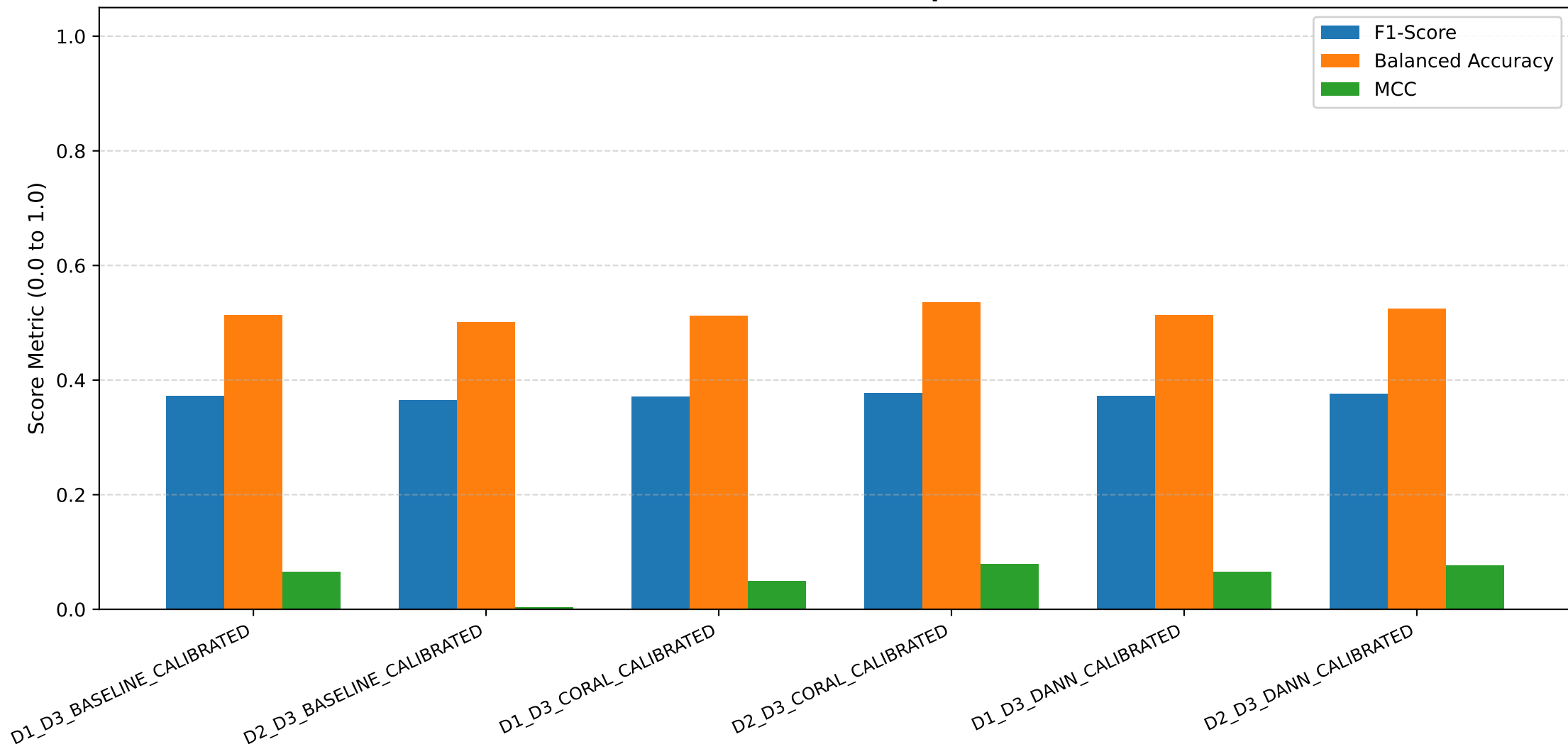
ARGUS Phase 3: Cross-Domain Transfer & Adaptation on IEC 60870-5-104 (D3)
