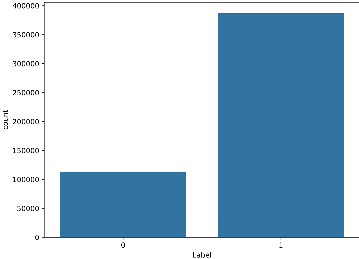
Target Distribution
