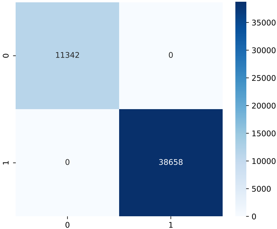
LightGBM - Confusion Matrix
