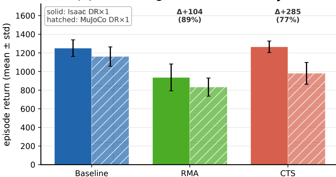
(C) Sim2Sim @ DR×1: Isaac vs MuJoCo
