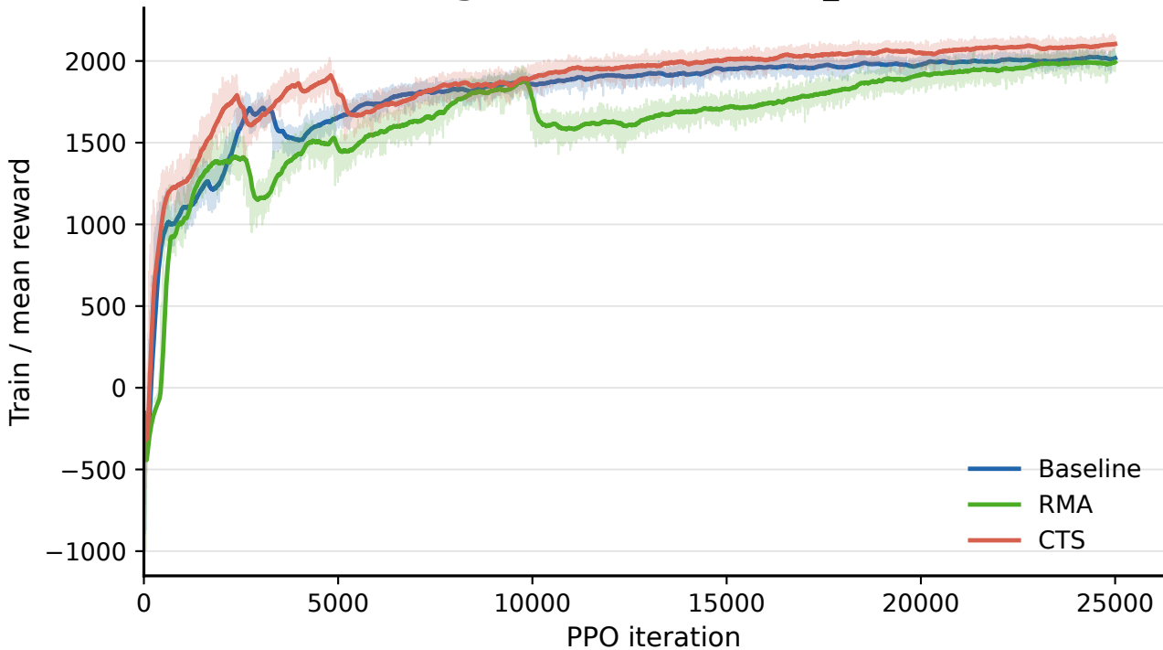
Go2 — PPO learning curve (Train/mean_reward, Z=8, FULL)
