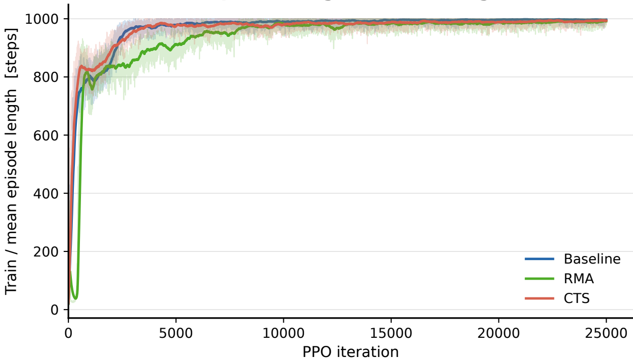
Go2 — Mean episode length over training (Z=8, FULL)
