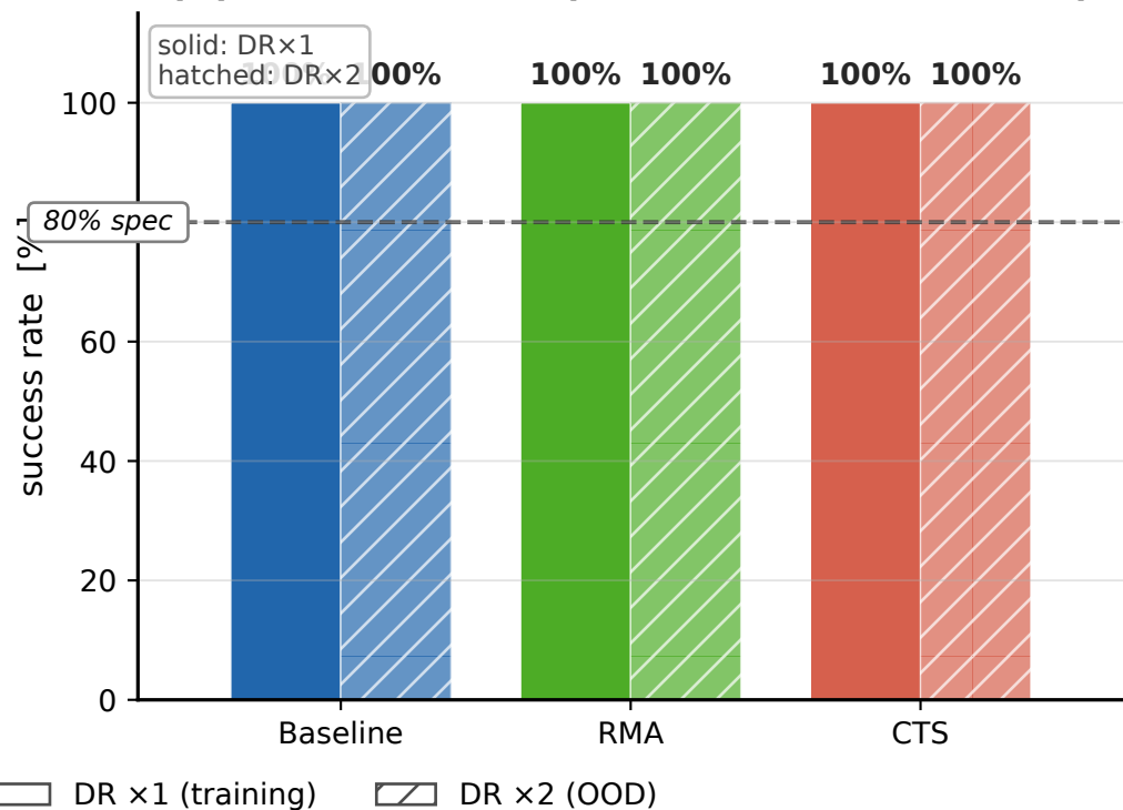
(B) Success rate (DR×1 vs DR×2 in Isaac)
