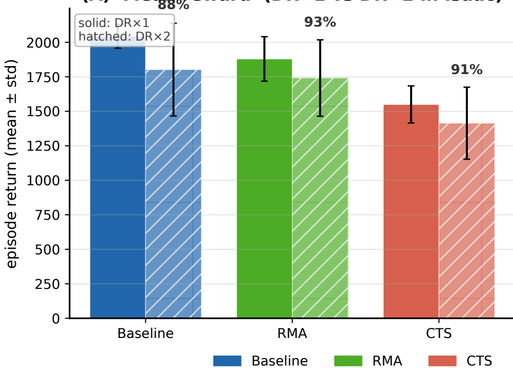
(A) Mean reward (DR×1 vs DR×2 in Isaac)
