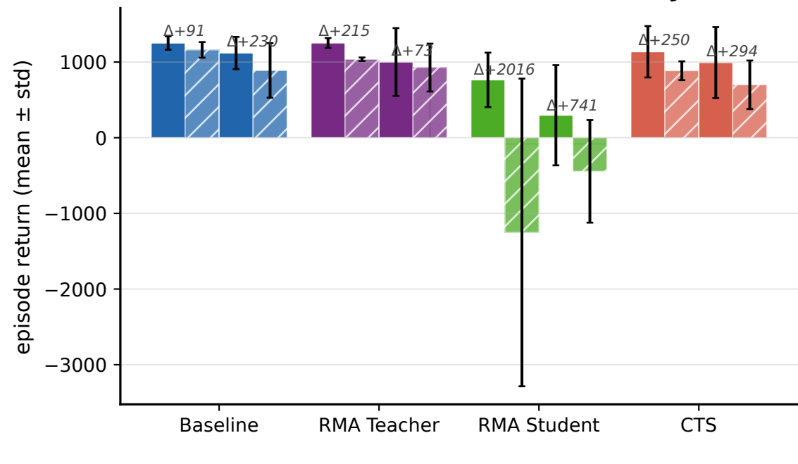
(B) Absolute reward — Isaac vs MuJoCo
