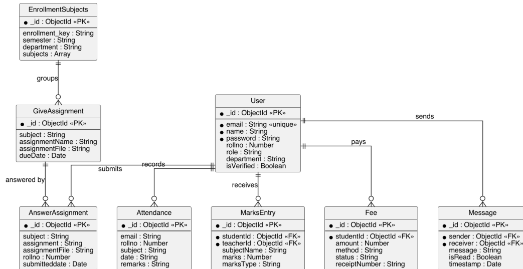
Figure 3.2: Entity-relationship diagram of CampusEase.
