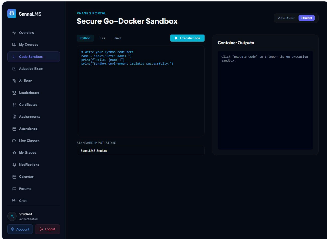
Code sandbox — run real code in the browser
