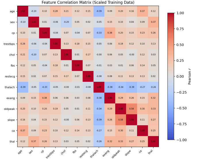
Fig. 2. Pearson correlation matrix of the thirteen clinical features. Edges of the feature graph are instantiated for entries with |r| \geq \tau = 0.15 ; the minimum spanning tree then adds the few bridges required for connectivity.
