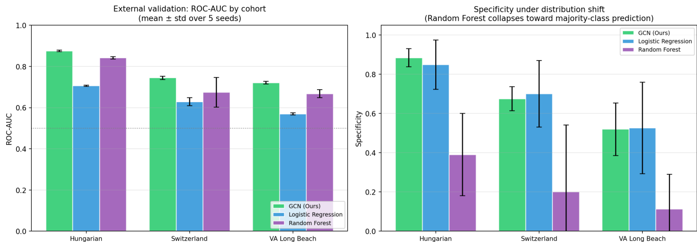
Fig. 12. External validation. Left: ROC-AUC by cohort for the transported models (mean±std over five seeds); the feature-node GCN leads on all three cohorts. Right: specificity under distribution shift; Random Forest degenerates toward majority-class prediction while the GCN retains a balanced operating point.
