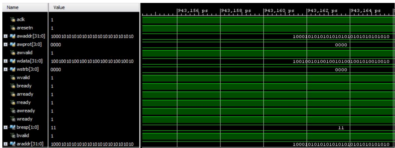
Fig. 7 AXI4 Protocol simulation
