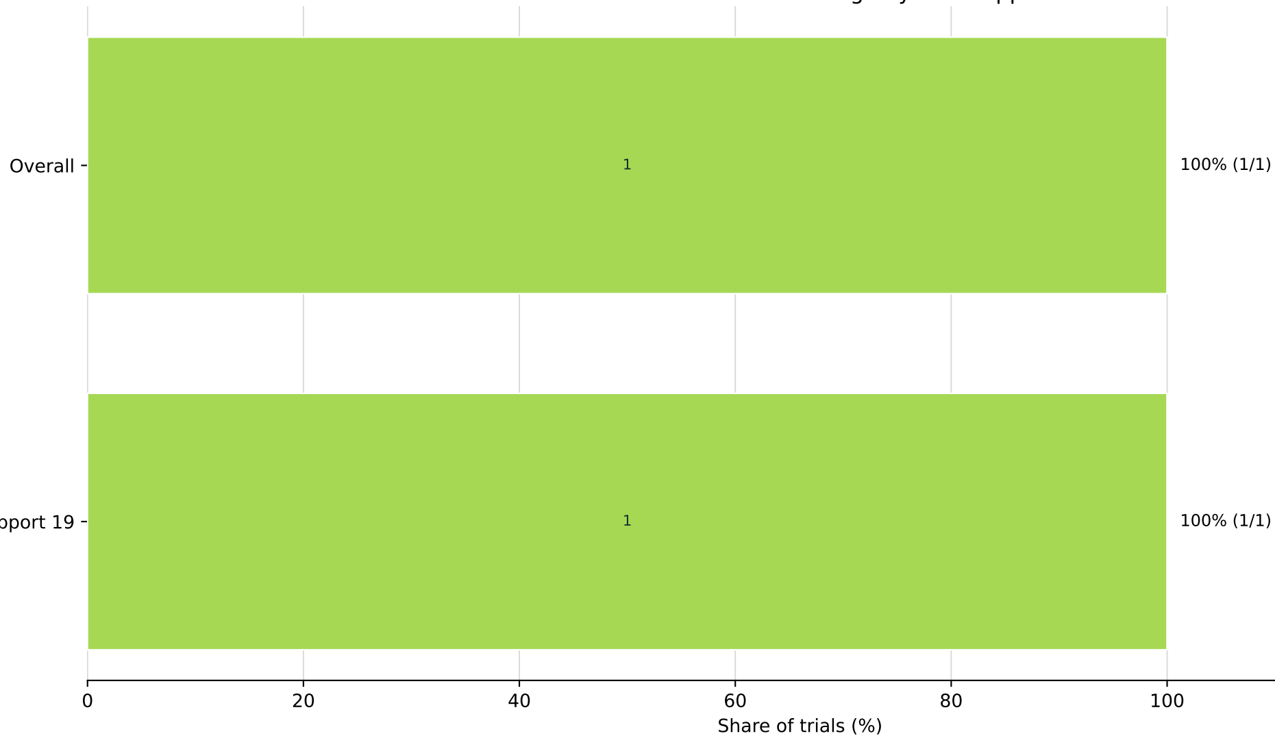
Dimension-selection coverage by true support
