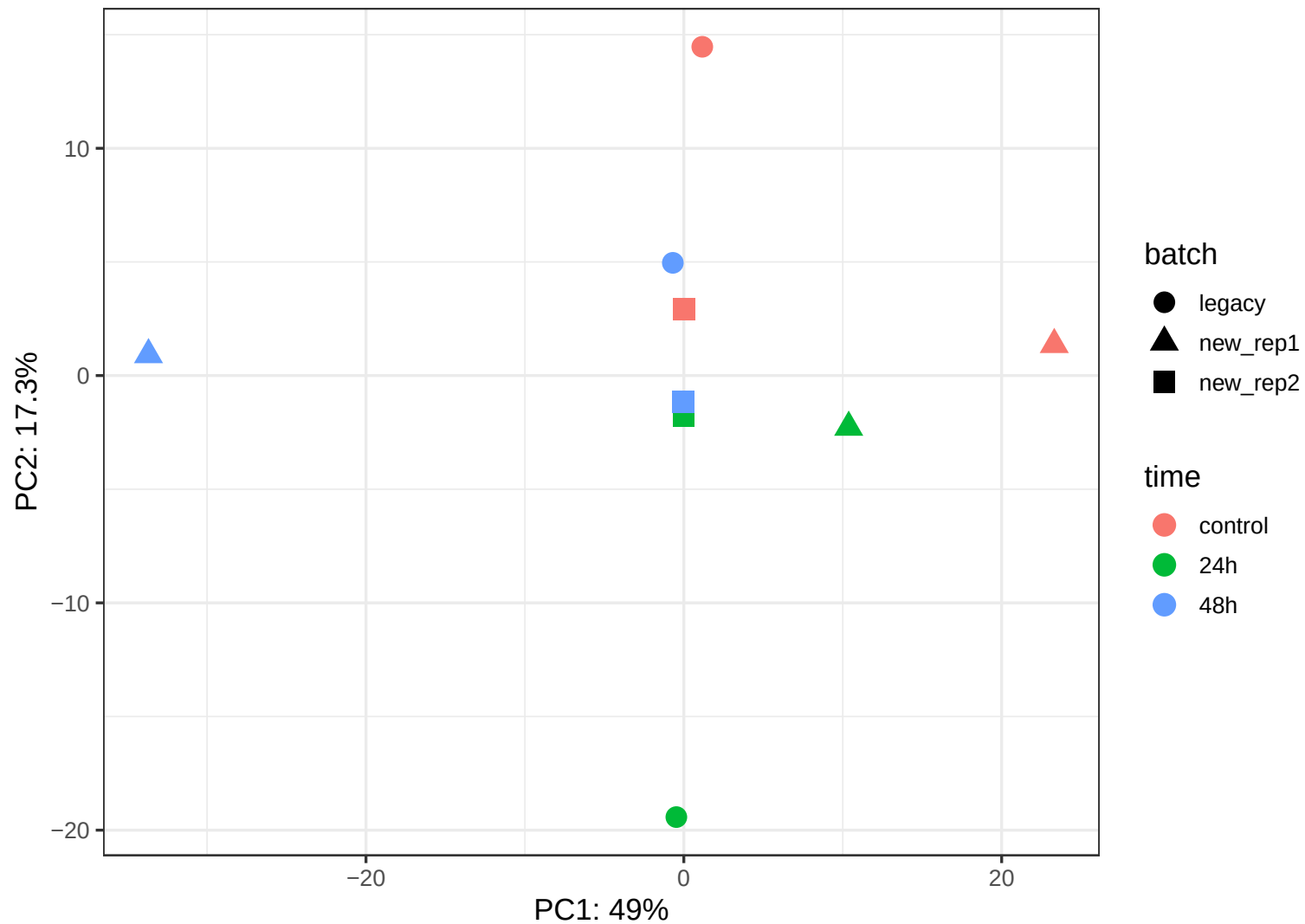
CLBMA PCA after limma::removeBatchEffect – coloured by time
