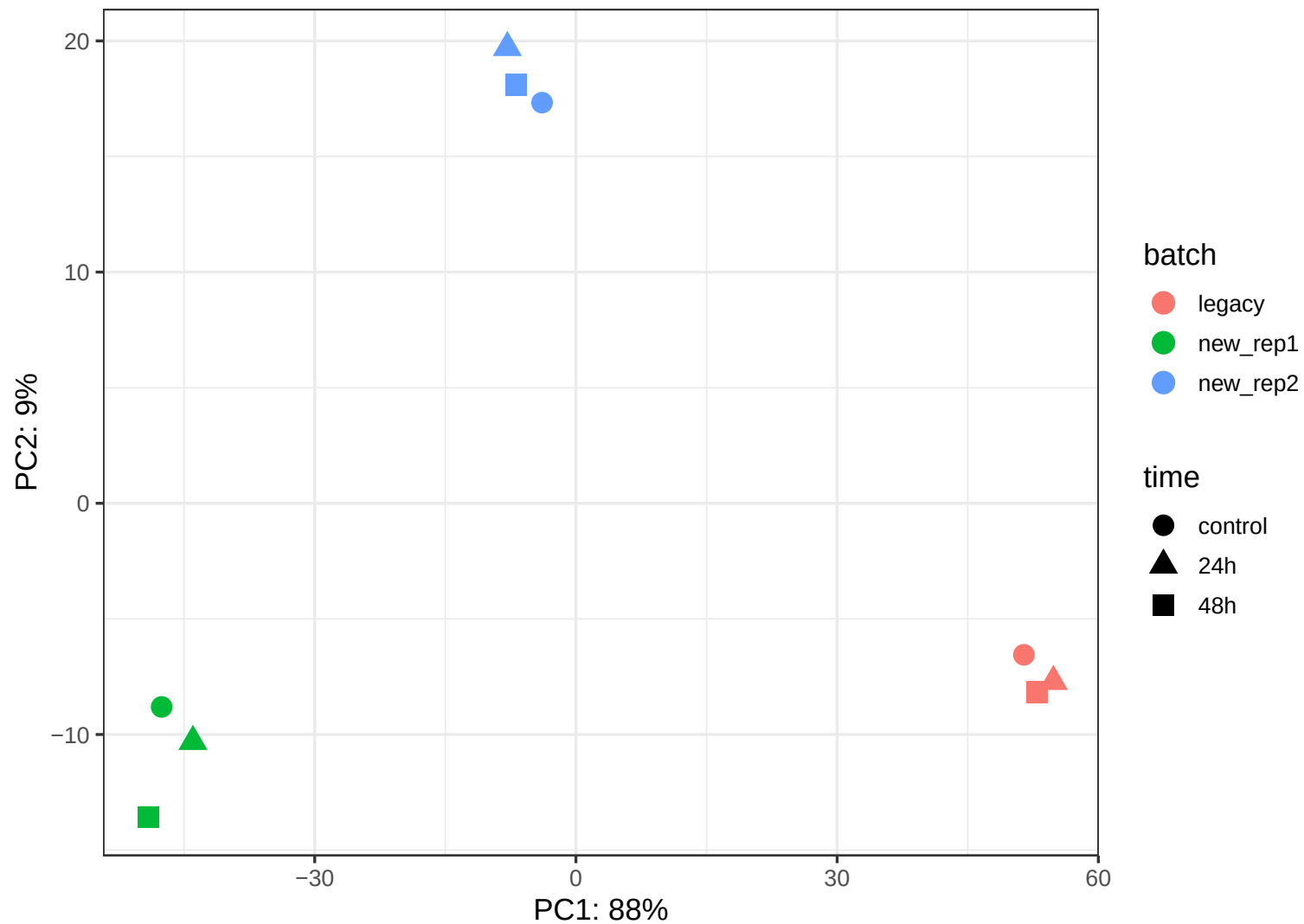
CLBMa ATAC-seq PCA (VST, blind) – coloured by batch
