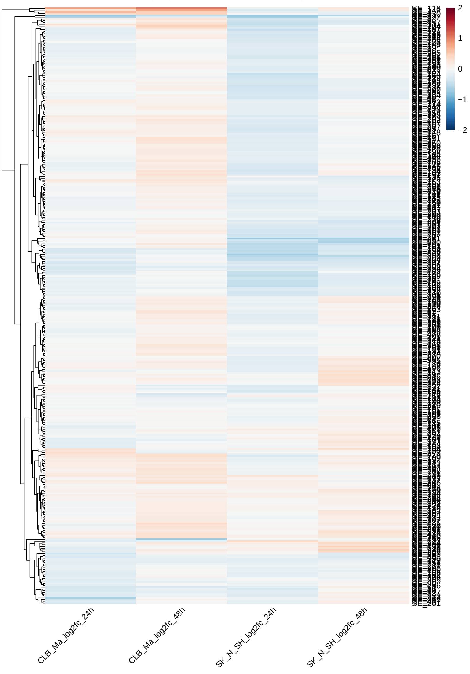
Super Enhancer Accessibility Changes (Log2 Fold Change vs Control)
