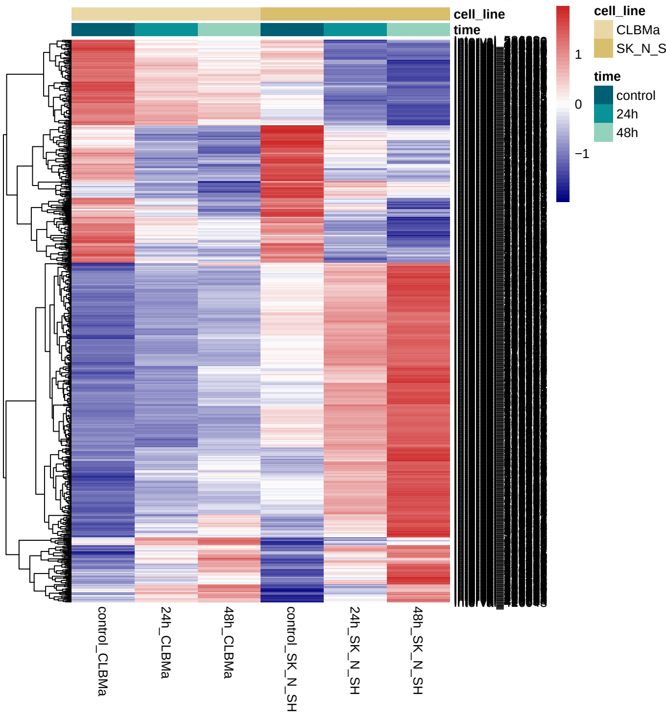
Heatmap of signif. All DARs 48h vs control (merged replicates).
