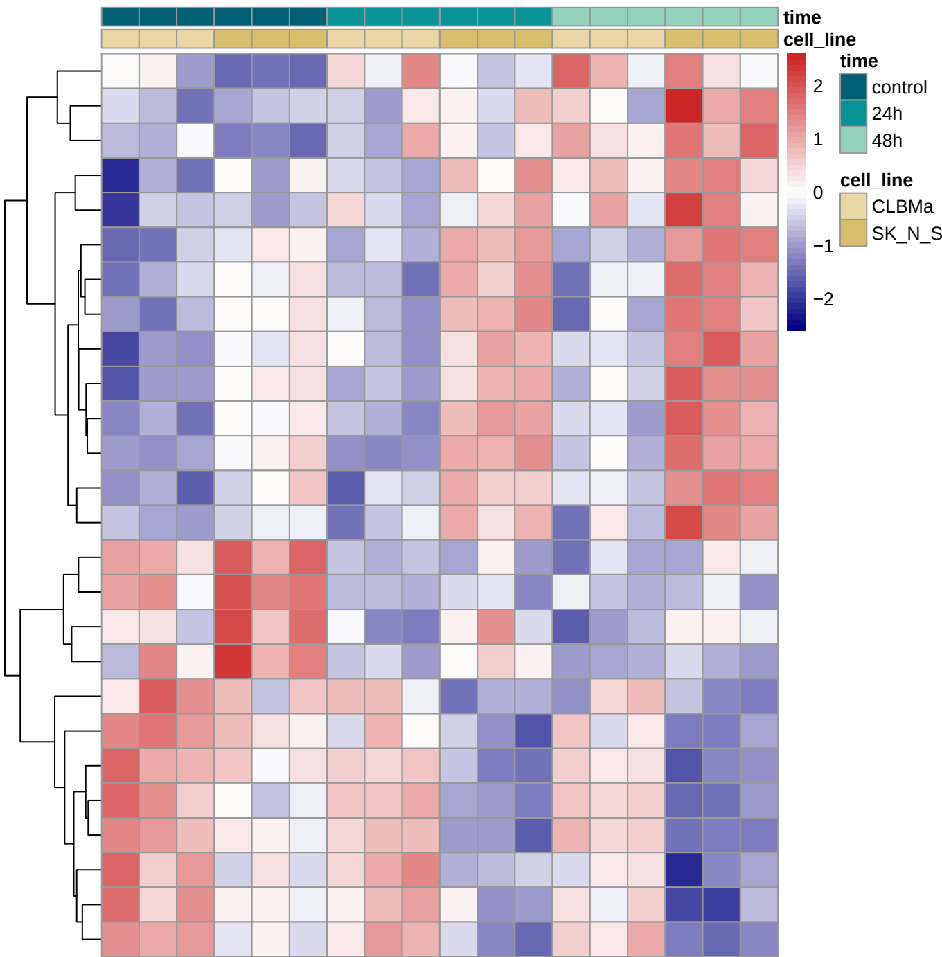
Heatmap of signif. DAR ADRN vs MES all DARs ADRN-specific genes only (defined by RNA-seq)
