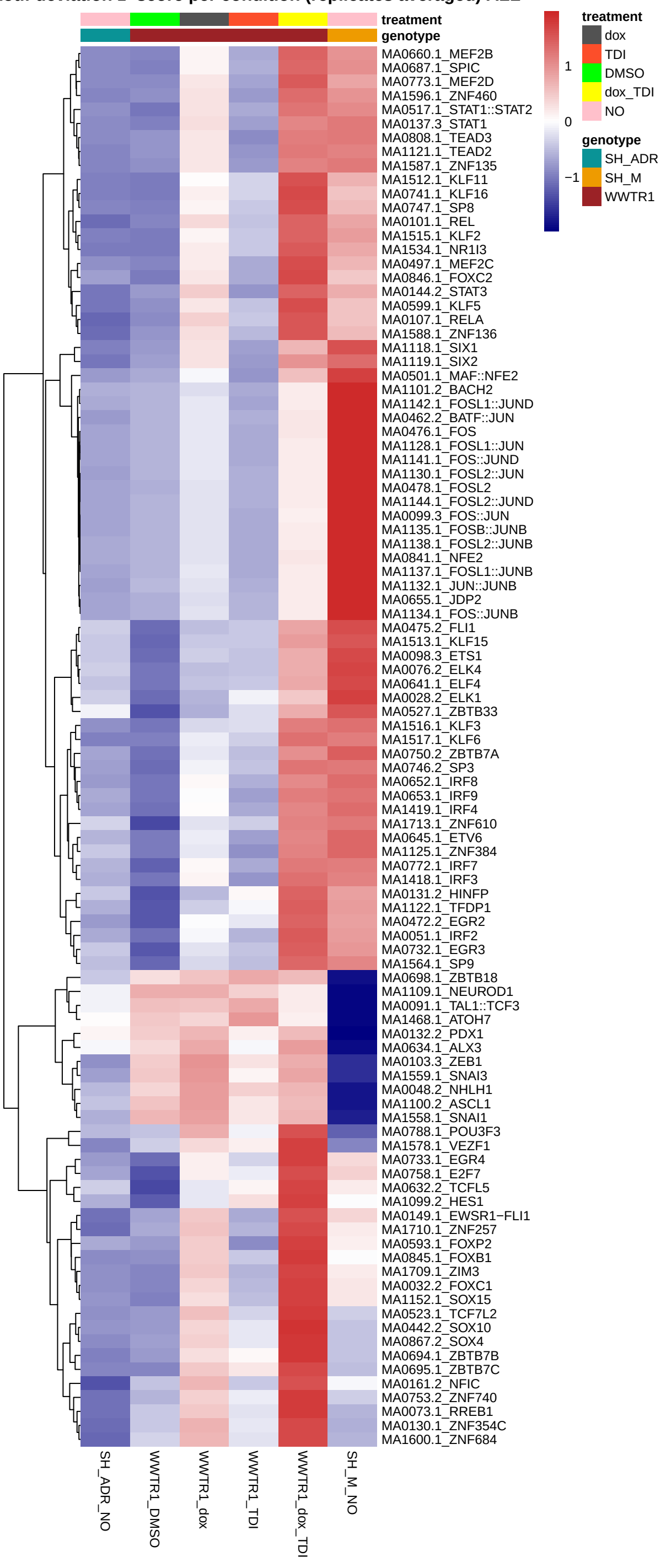
motif deviation z-score per condition (replicates averaged) ALL
