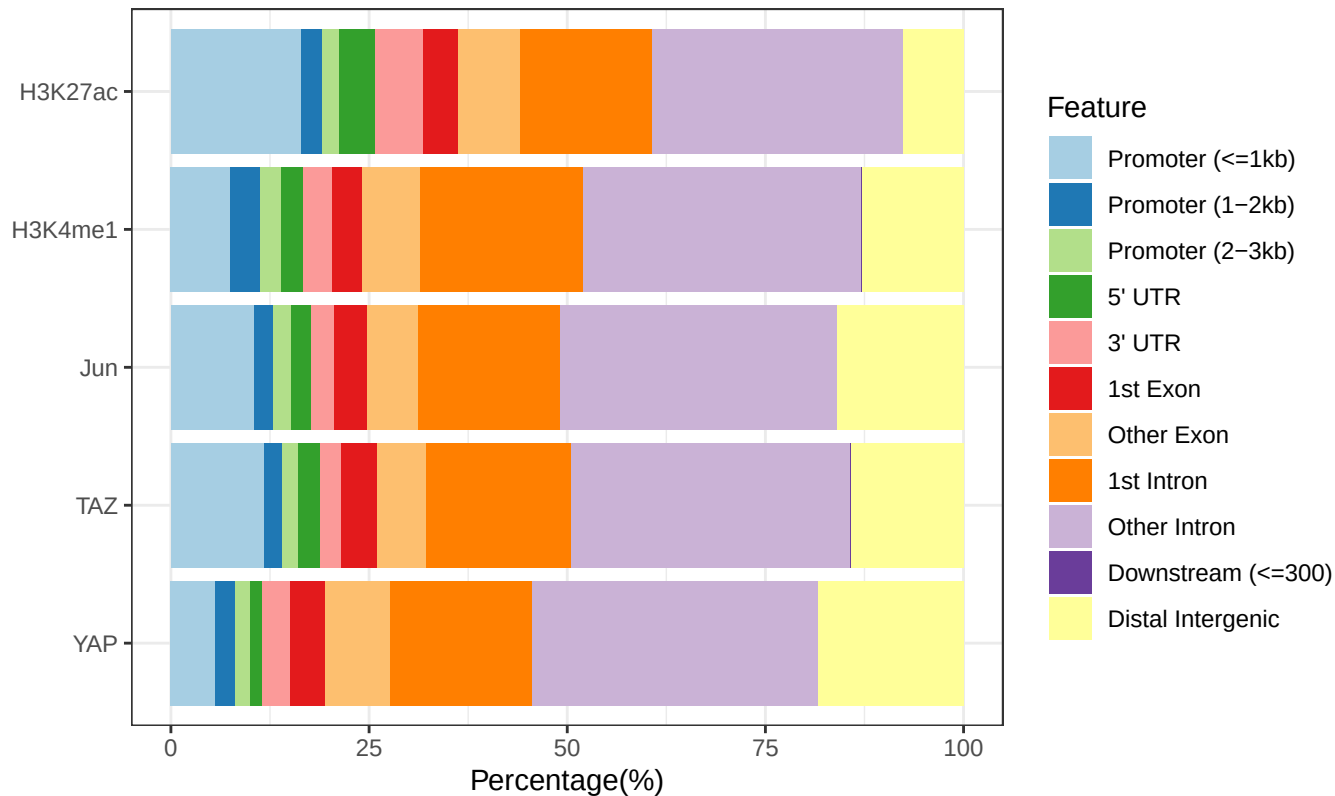
Feature Distribution
