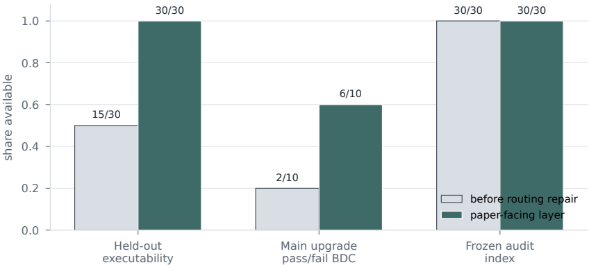
Routing repairs improve executability without rewriting the frozen index
